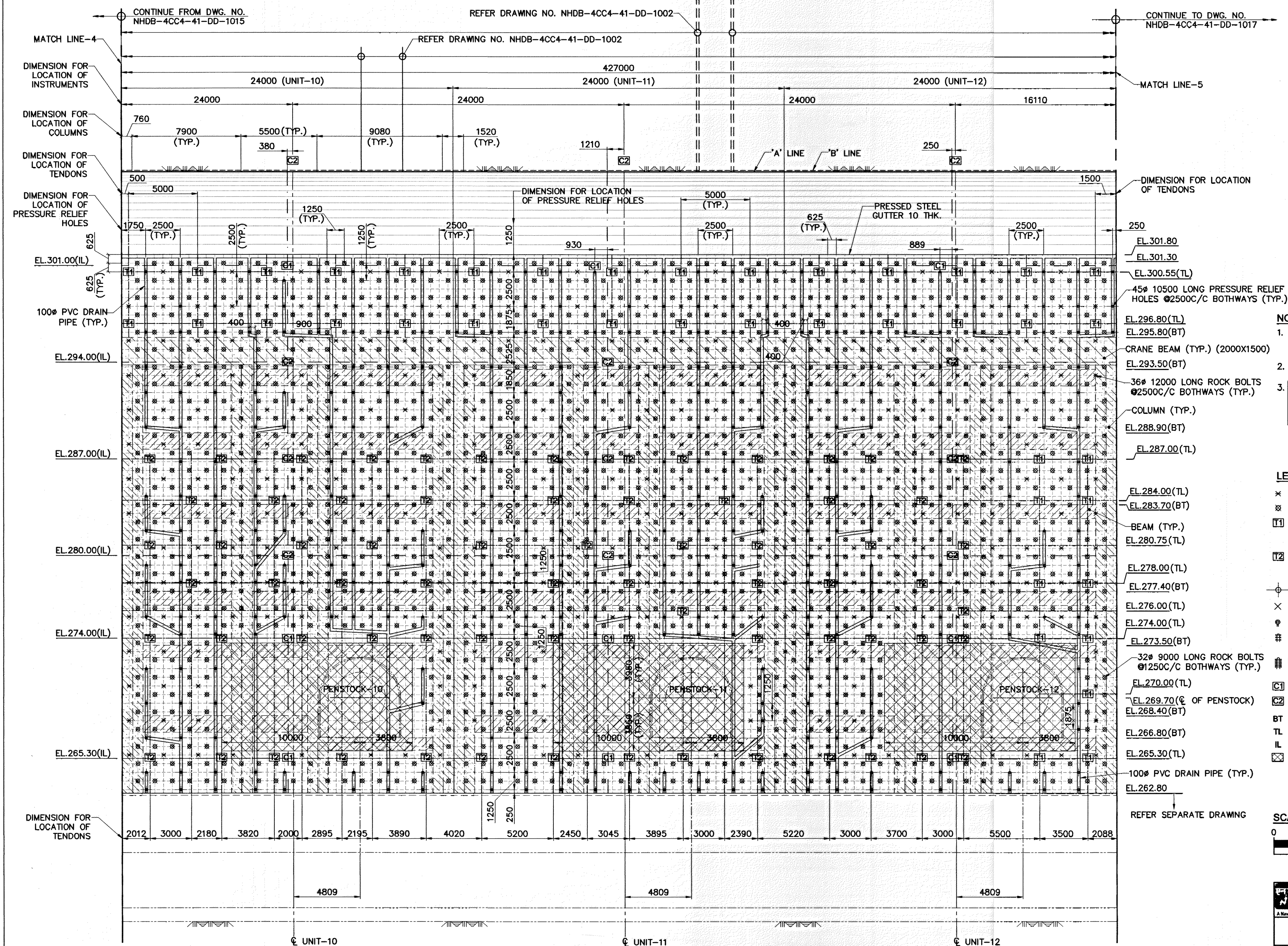
ELEVATION - UPSTREAM WALL (TYPICAL ARRANGEMENT)
